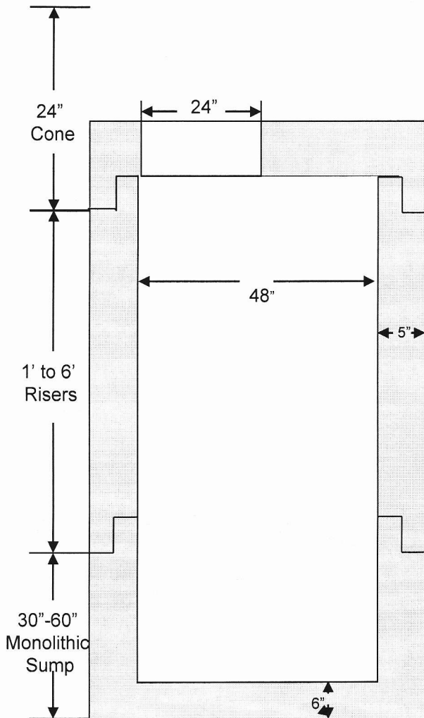
Section View - Typical Installation
