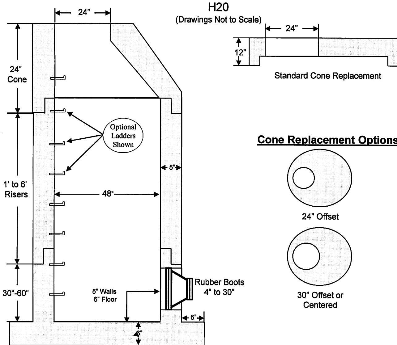
Section View - Typical Installation
