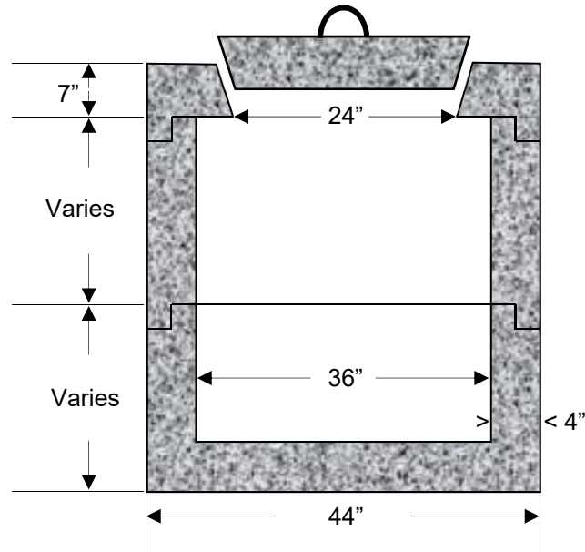
Section View - Typical Installation
