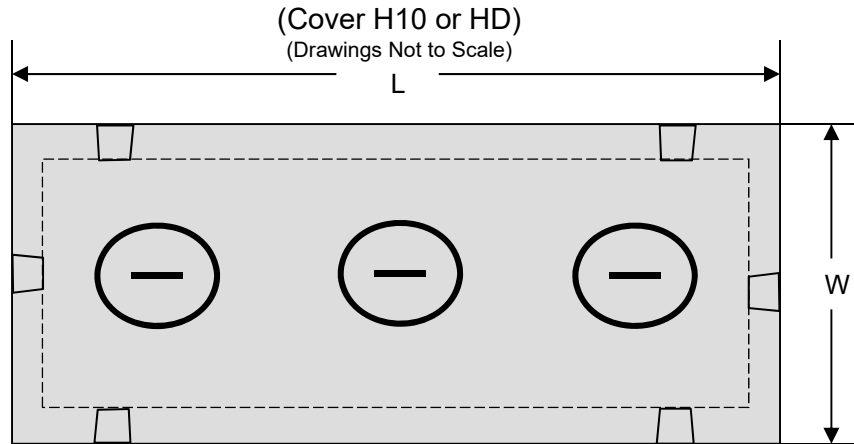
TOP VIEW-TOP 3 CLEANOUTS - 26" DIAMETER
