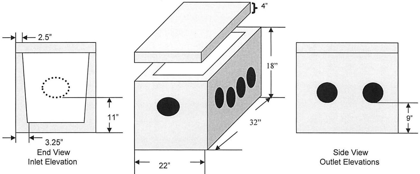
H10 Schematic: H10 cover 2": H20 cover 3"
