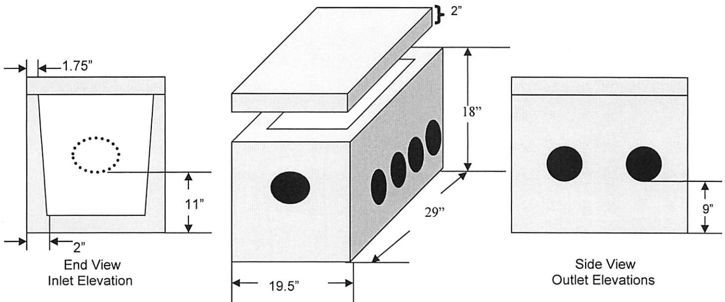
H20 Schematic: H10 cover 2": H20 cover 3"
