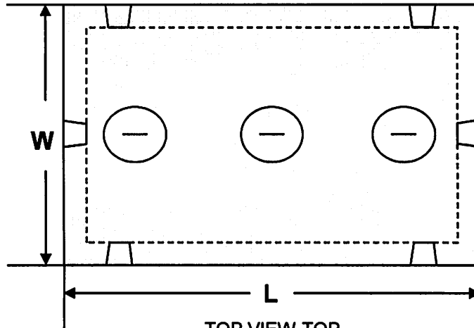
TOP VIEW-TOP 3 CLEANOUTS - 26" DIAMETER min.
