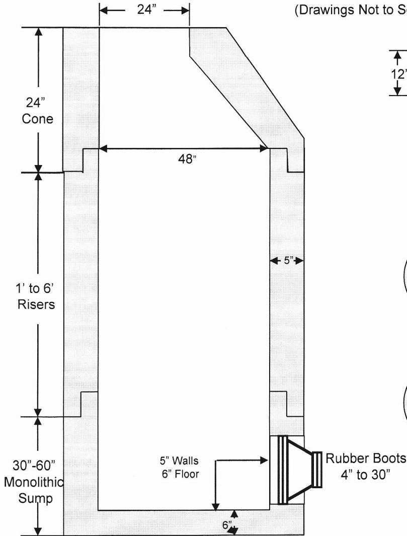
Section View - Typical Installation
