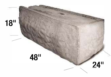
90 Degree Return Boulder 48 x 18 x 24 Weight: 1100 lbs. Sq. Ft. / Block: 6 sq. ft.
