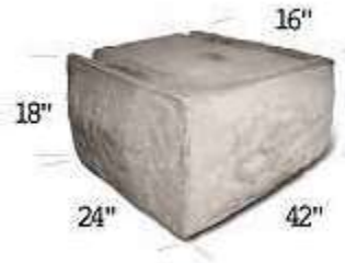
1/2 Corner Boulder 24" x 18" x 42" (16") Weight: 900 lbs. Sq. Ft. / Block: 3 sq. ft.
