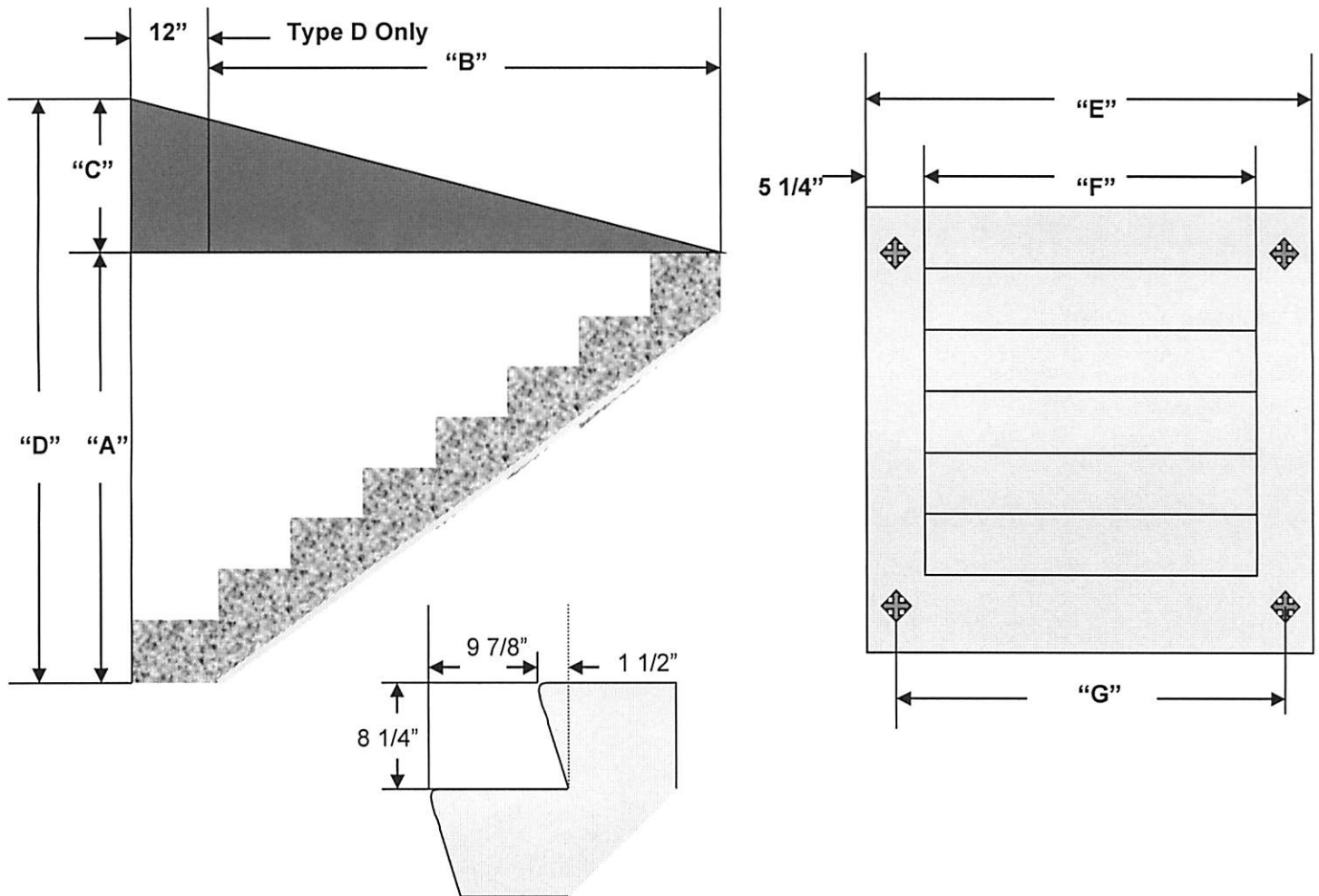
Detail of Tread and Rise
