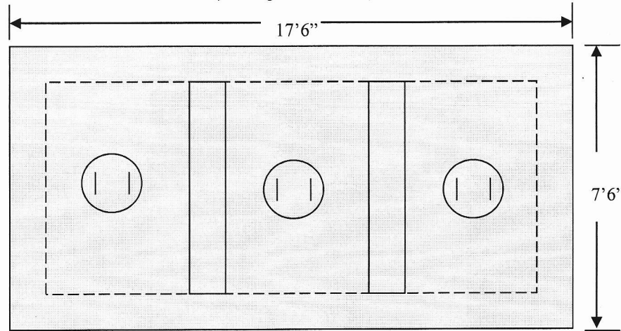
TOP VIEW-TOP 3 CLEANOUTS - 26" DIAMETER
