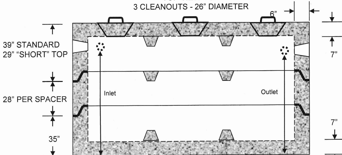
CROSS SECTION VIEW WITH ONE SPACER TAPERED CROSSMEMBERS
