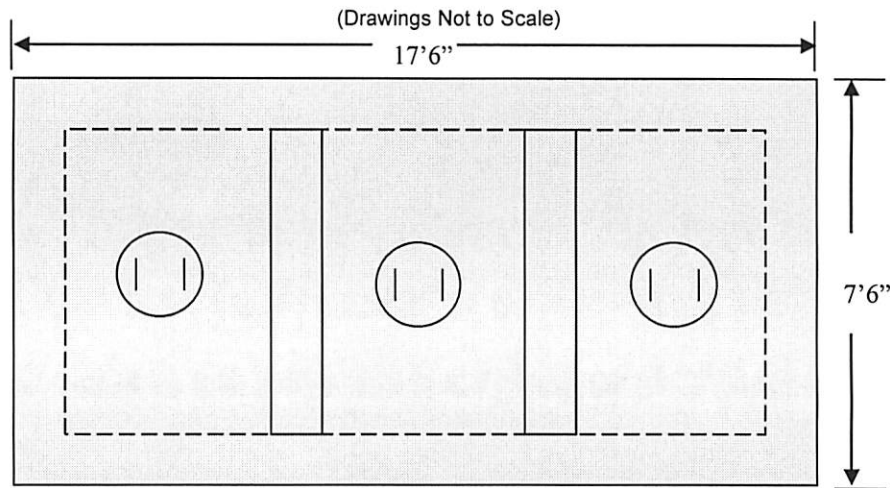
TOP VIEW-TOP 3 CLEANOUTS - 26" DIAMETER
