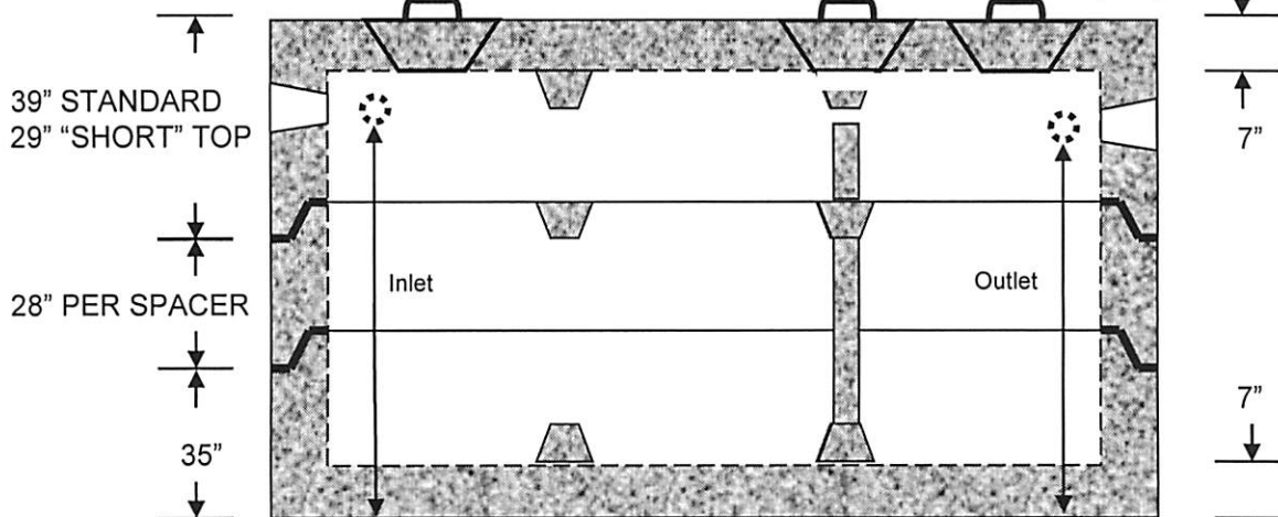
CROSS SECTION VIEW WITH ONE SPACER TAPERED CROSSMEMBERS
