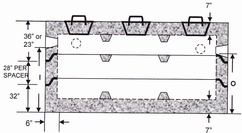
CROSS SECTION VIEW WITH ONE SPACER TAPERED CROSSMEMBERS
