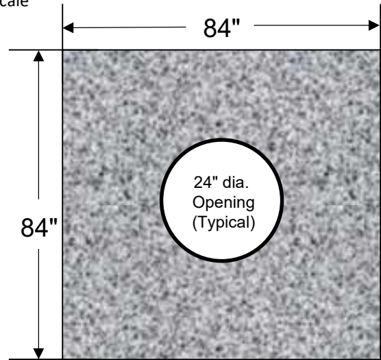
Top View-Cover
