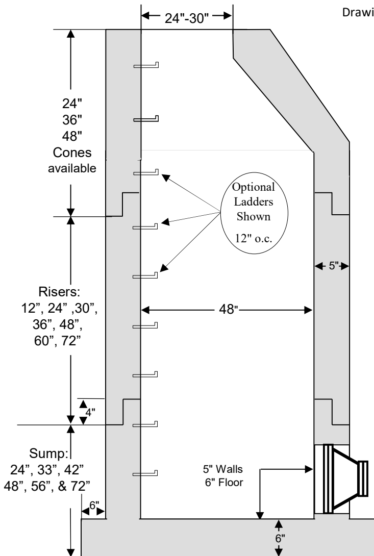
Section View - Typical Installation
